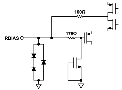
Figure 41. Equivalent RBIAS Input/Output Circuit
